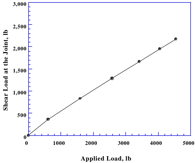
Figure 4. Applied Load vs. Shear Load in Test No. 1
