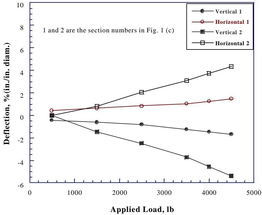
Figure 5 Applied Load vs. Deflection at the Loading Point in Test No. 1
