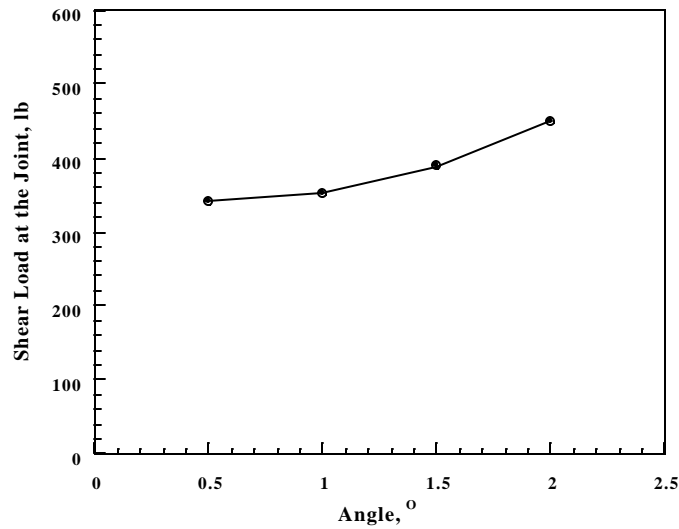
Figure 6. The Relationship between Angle and shear Load in Test 2
