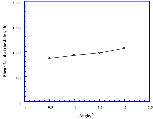
Figure 3. The Relationship between Angle and shear Load in Test No. 1
