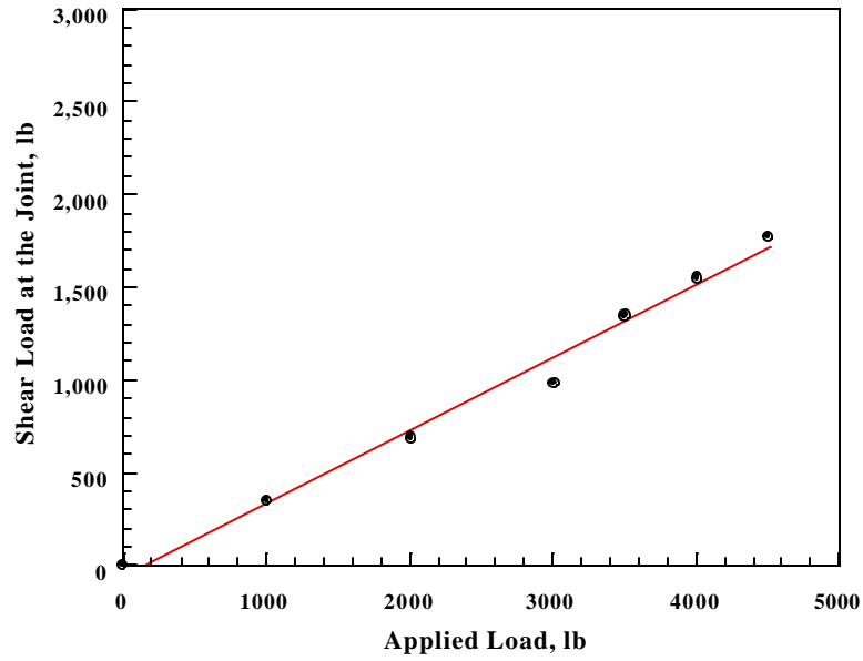
Figure 7. Applied Load vs. Shear Load in Test 2
