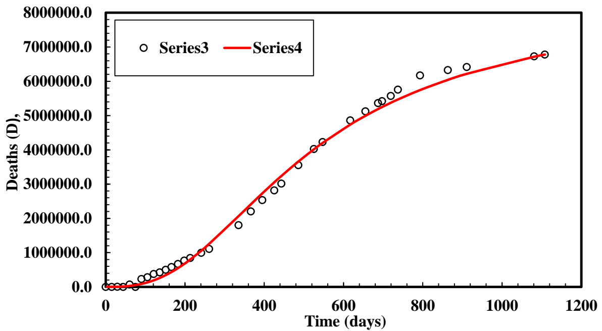
Figure 2. Vipulanandan Model Prediction of Total Deaths with Time (a) World and (b) United States of America
