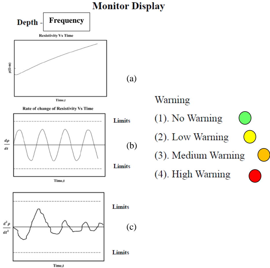
Figure 11. Variation of Total and Rates of Electrical Resistivity with Time at Various Depths
