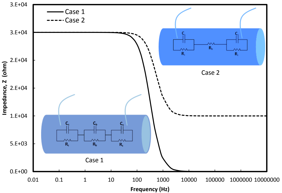
Figure 1. Vipulanandan impedance-frequency models for composite materials
