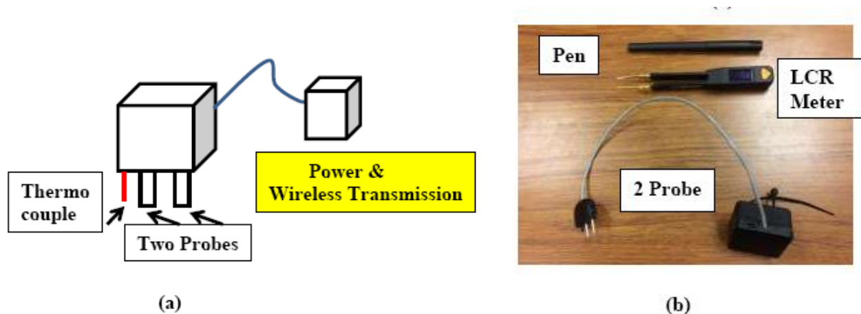
Figure 9. Two Probe Monitoring with Wireless Transmission (a) Schematic and (b) Actual Device (SensyRoc), two probe pocket LCR and a Pen.
