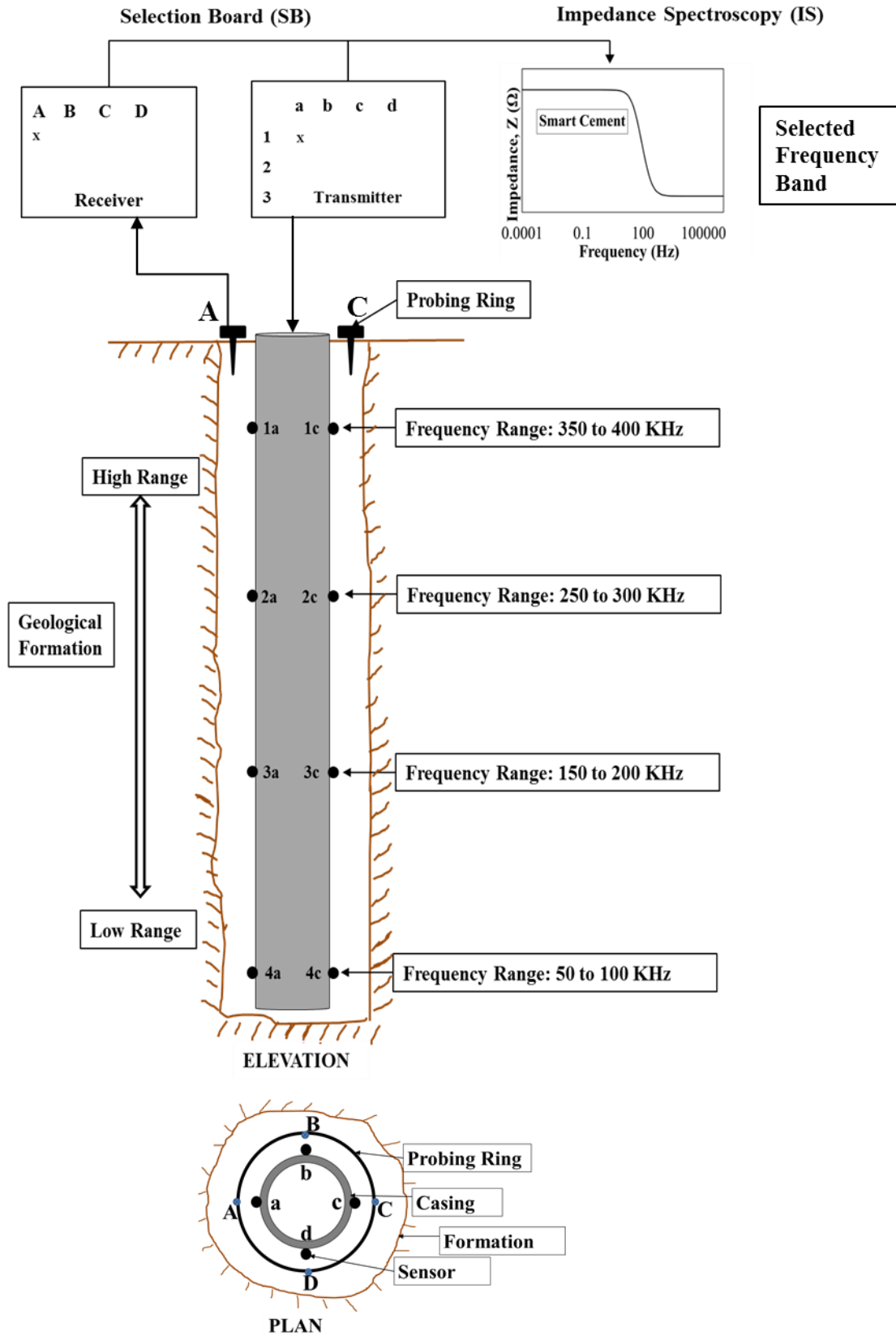
Figure 10. Schematic Configuration of the Field Oil Wells and Piles to be Installed
