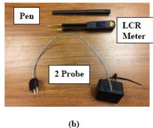
Figure 9. Two Probe Monitoring with Wireless Transmission (a) Schematic and (b) Actual Device (SensyRoc), two probe pocket LCR and a Pen.
