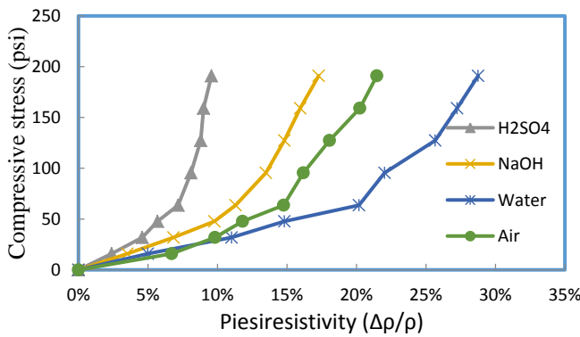
Figure 3: Compressive behavior of ultra fine cement
