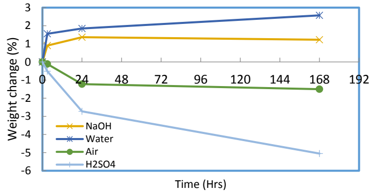
Figure 2: Weight change with time for fine cement
