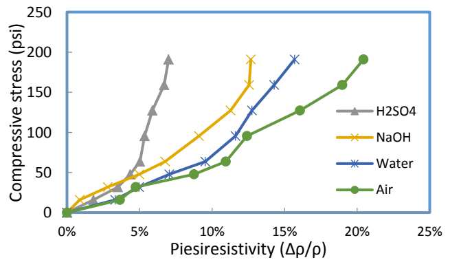
Figure 4: Compressive behavior of Portland cement
